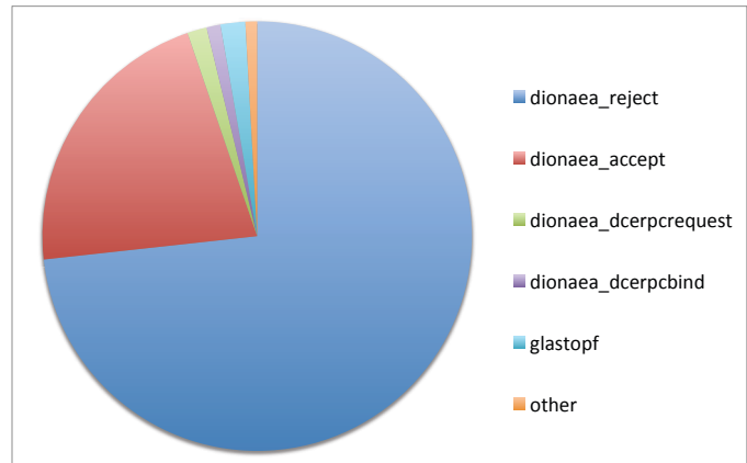
Fig. 3: Attack Features for Hosts with ThreatIndex \in [1.0, 50.0)
